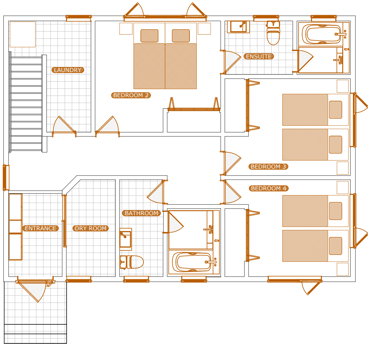
1st FLOOR
