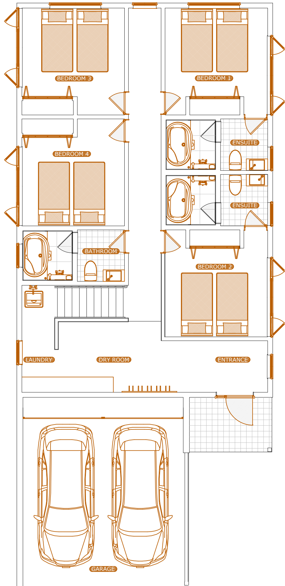
1st FLOOR
