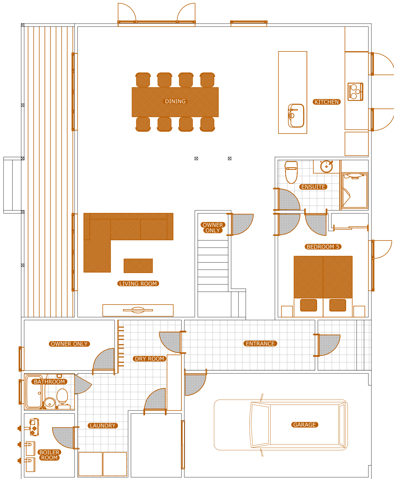
1st FLOOR
