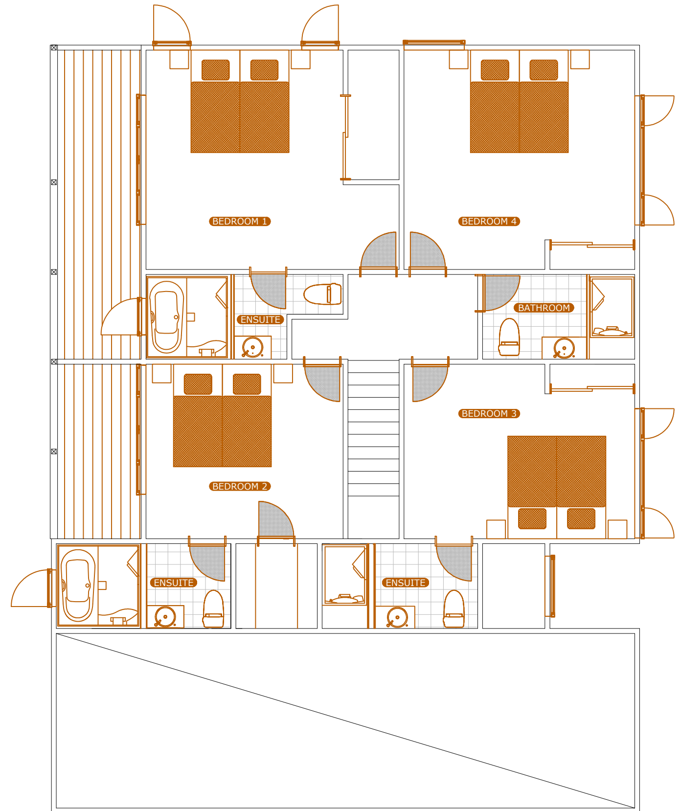
2nd FLOOR
