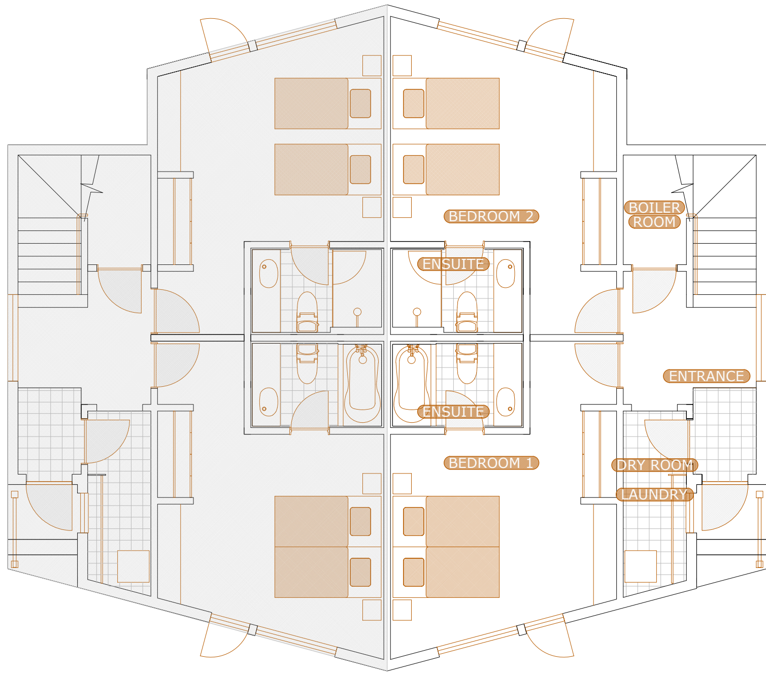
1st FLOOR
