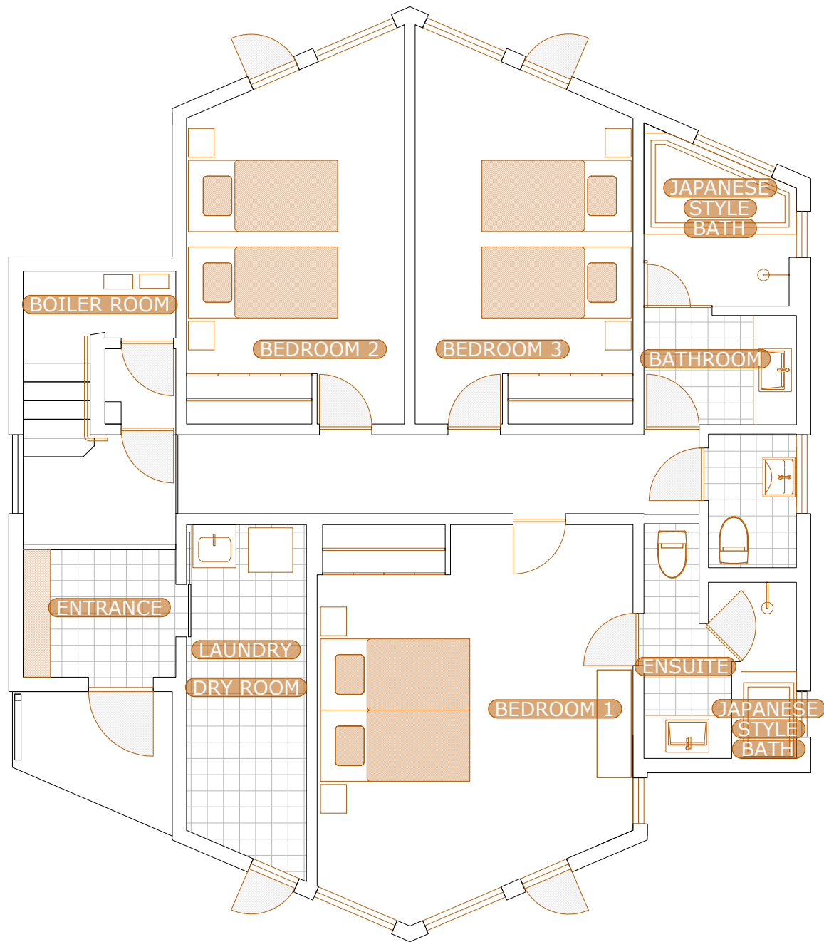
1st FLOOR
