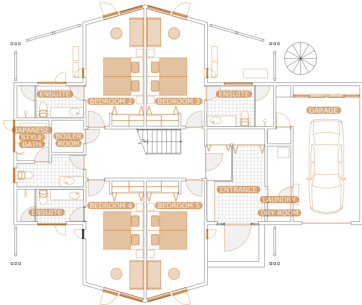
1st FLOOR
