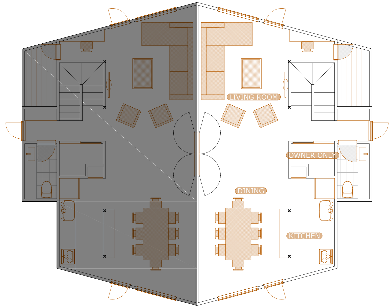
2nd FLOOR
