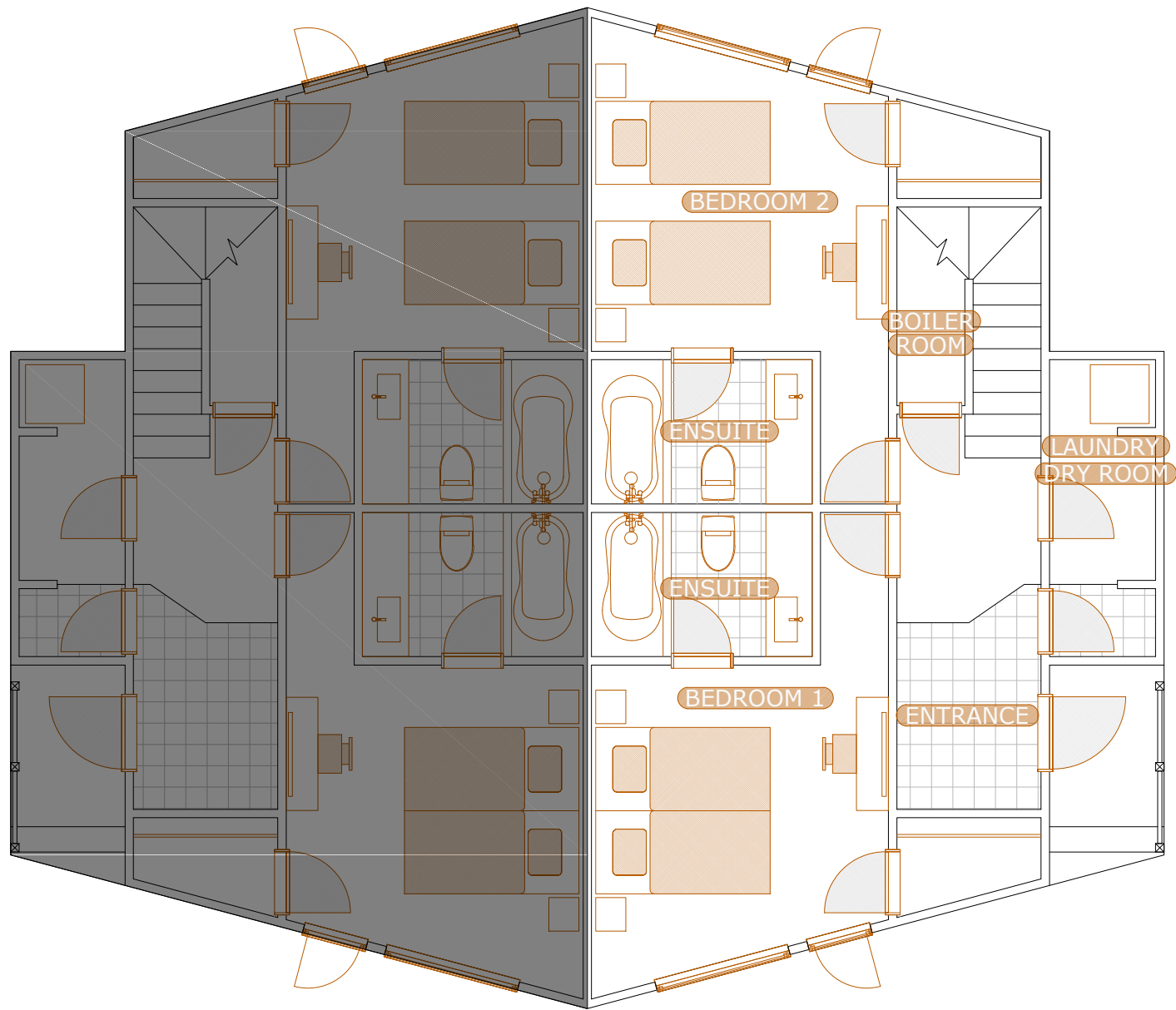
1st FLOOR
