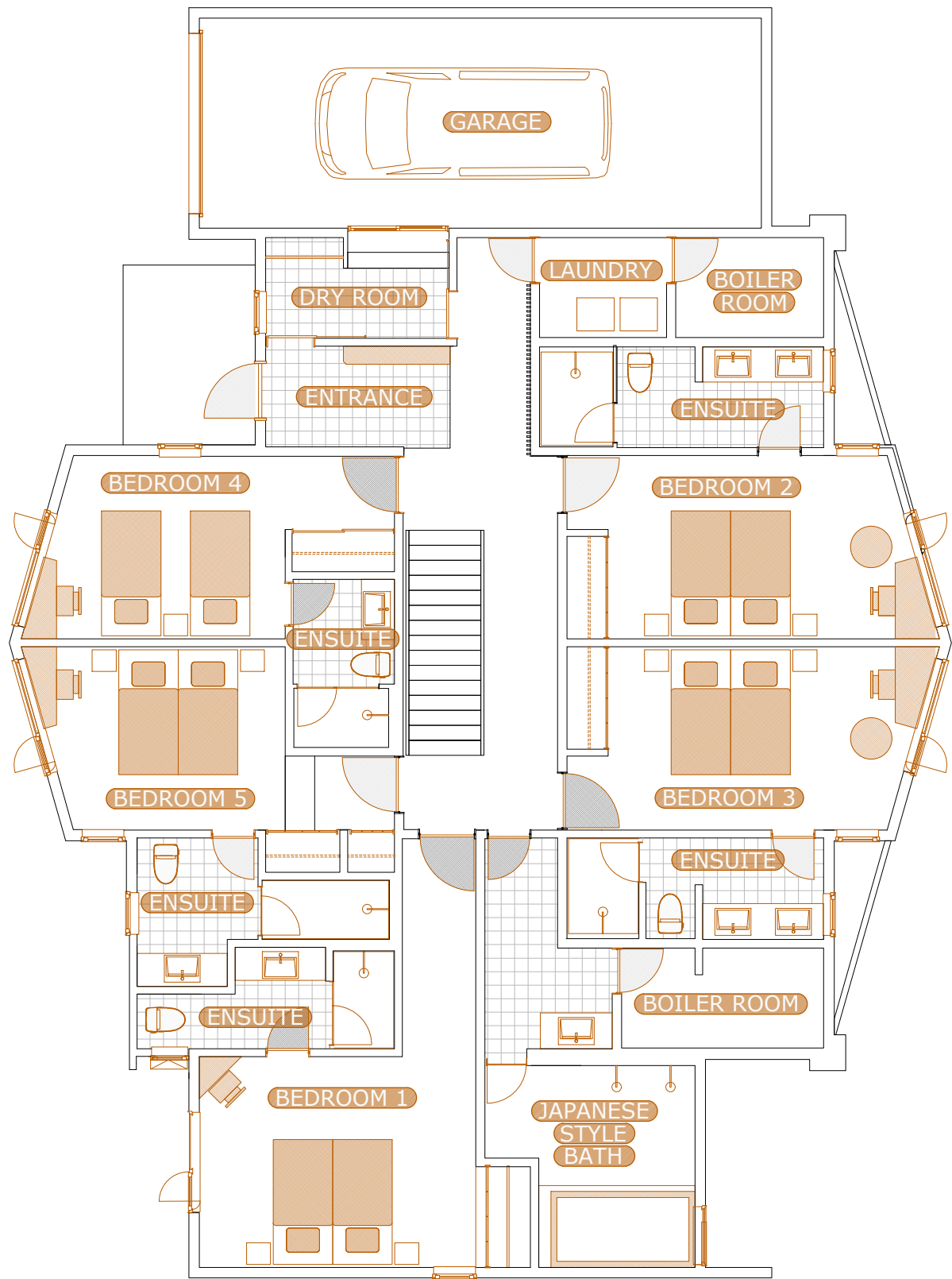
1st FLOOR
