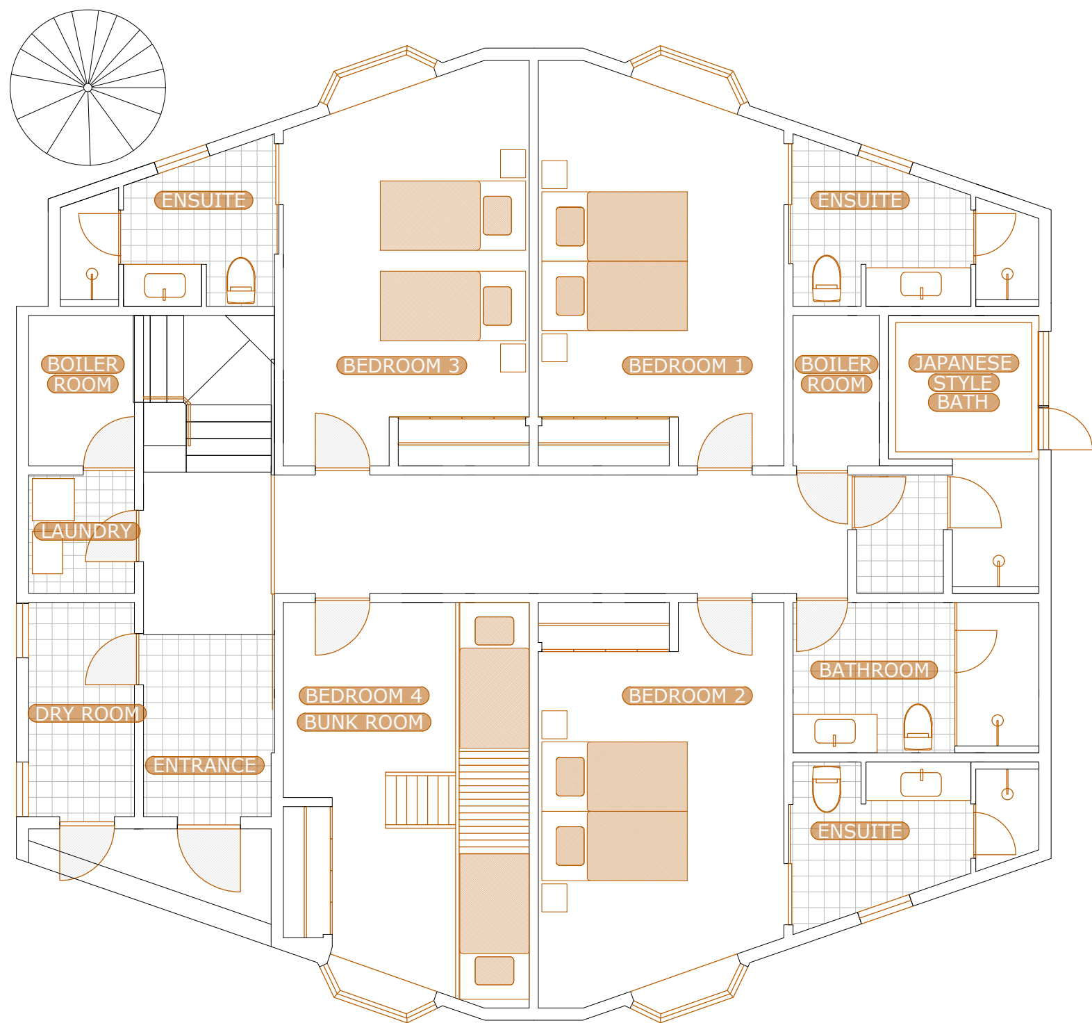
1st FLOOR
