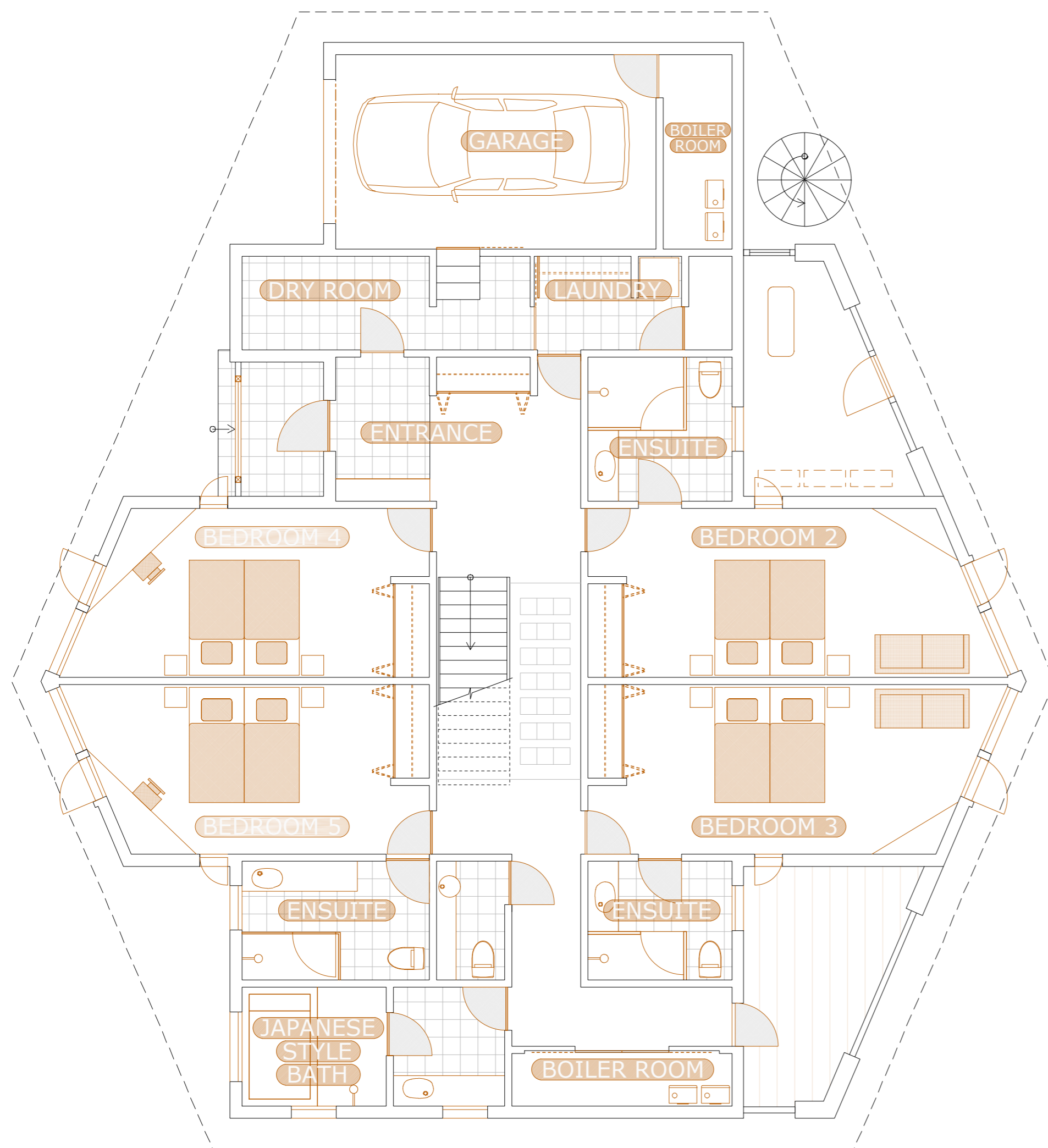
1st FLOOR
