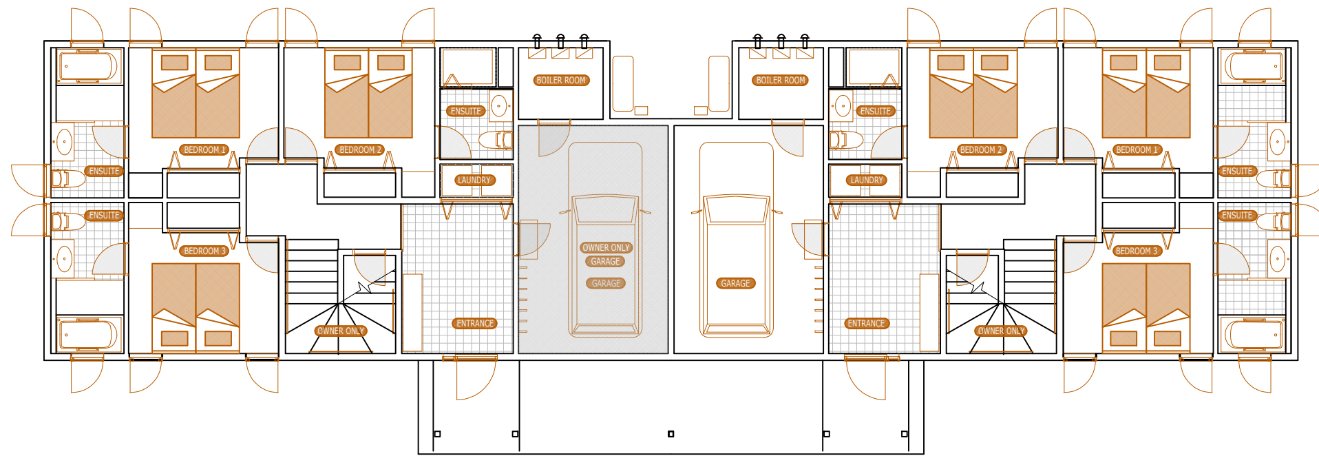
1st FLOOR
