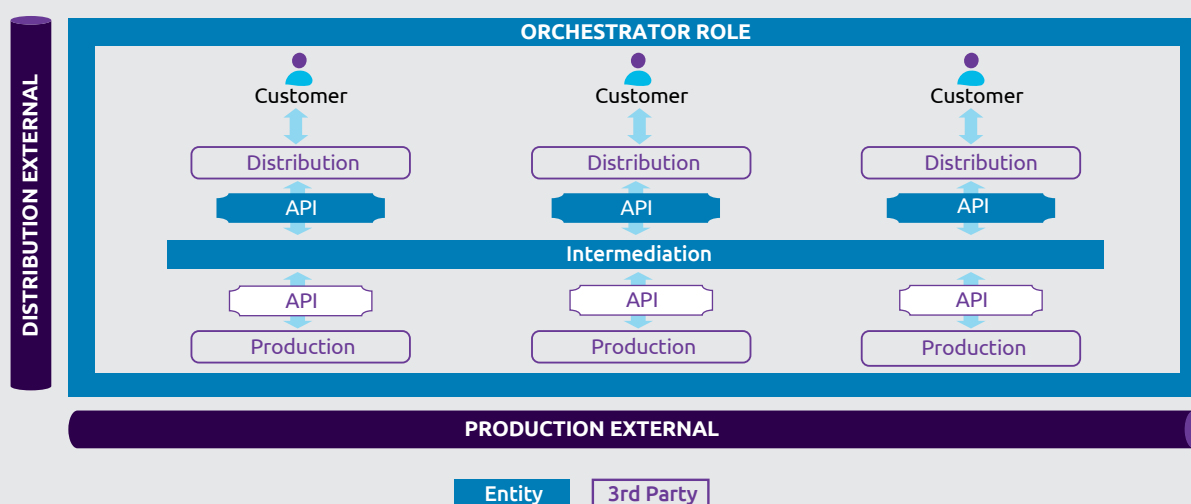
Figure 13. Orchestrator Role
