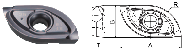
Fig.1(主刃・低抵抗形) (Main blade for low cutting force)
