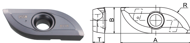
Fig.4(副刃・肉盛り加工用) (Sub blade for welding & hardened material)
