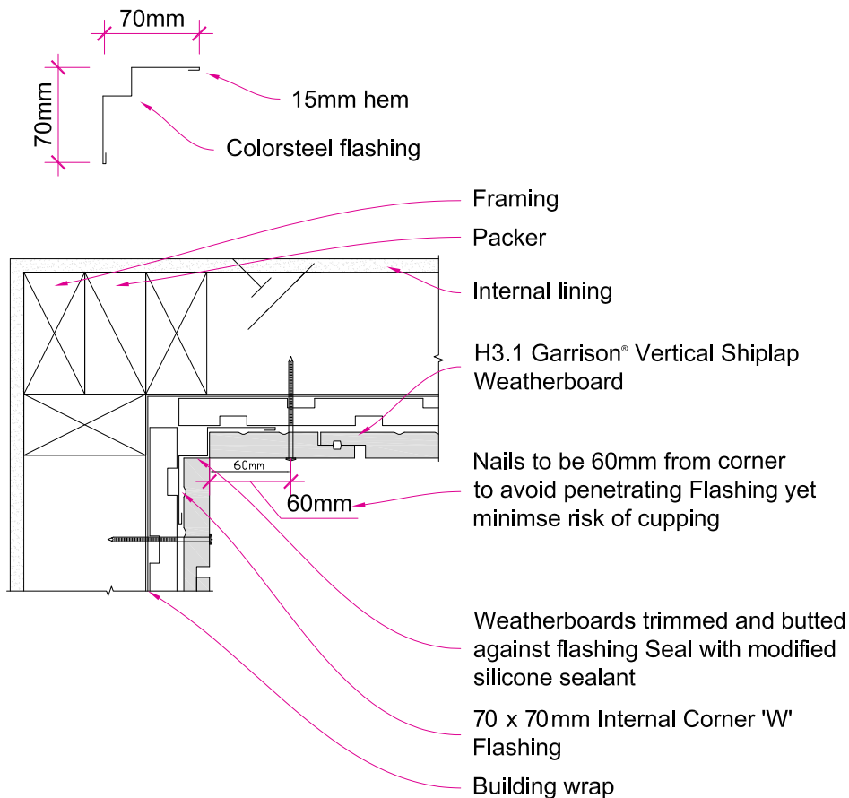
Figure 1.24 Cavity fixed – internal corner – w flashing
