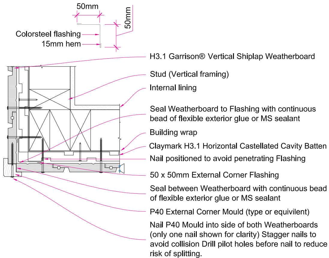
Figure 1.18 Cavity fixed – door jamb
