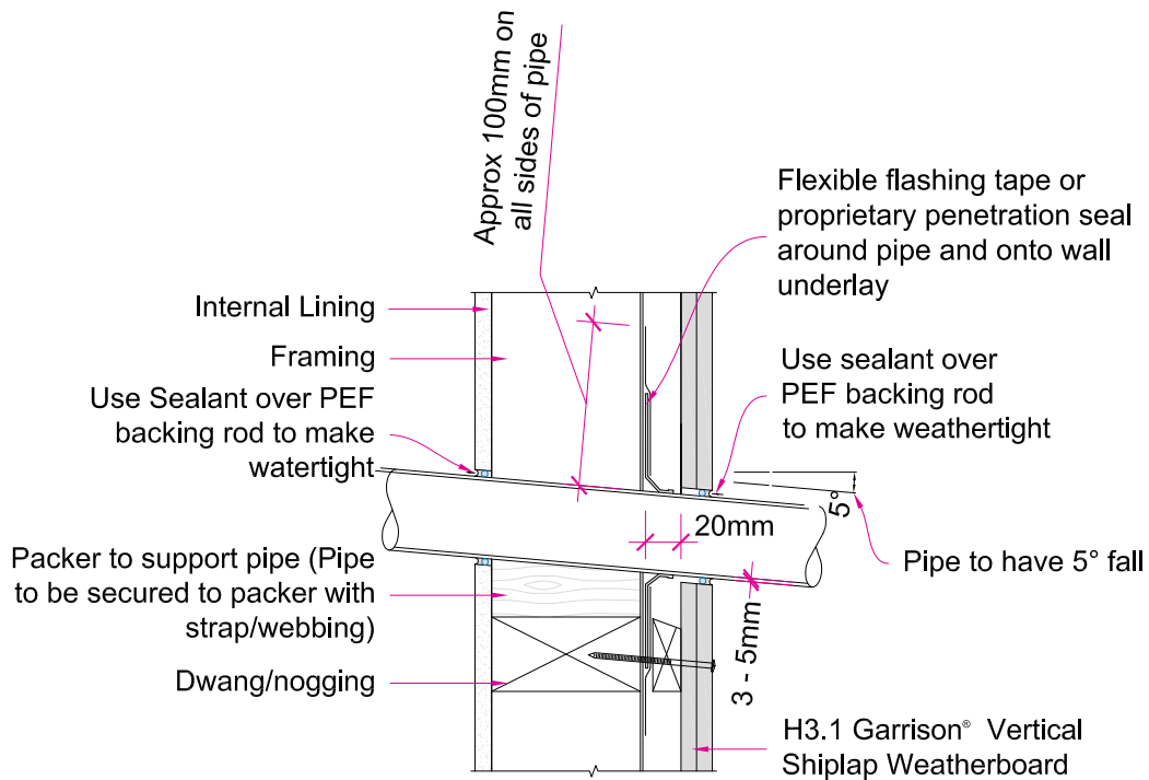
Figure 1.08 Cavity fixed – pipe penetration
