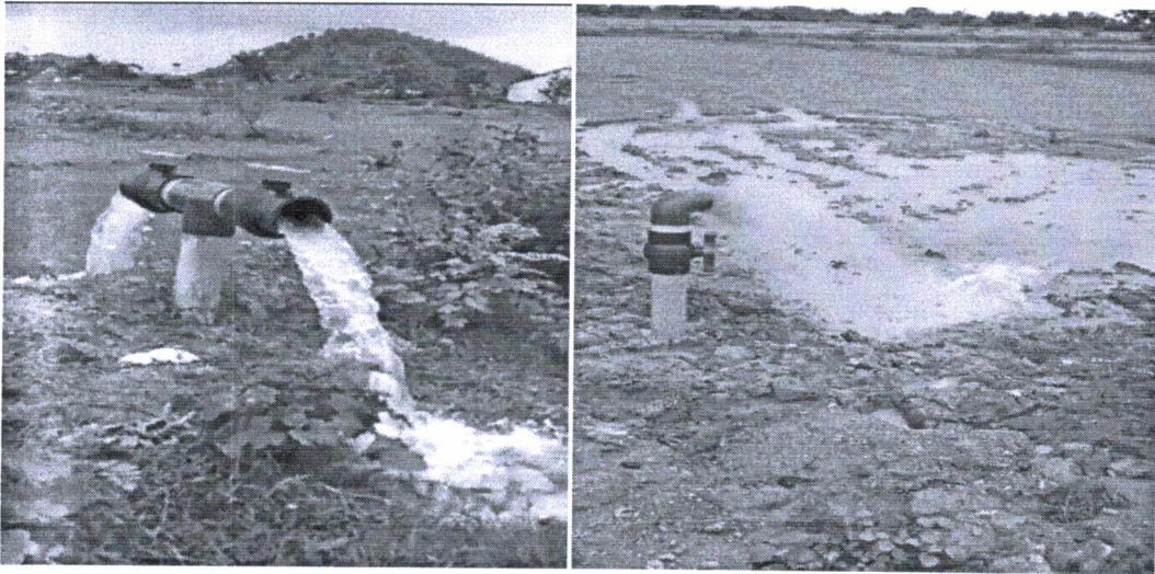
Under Ground Pipe Line Testing for Kharif water supply through single & double outlet Some of photographs during plantation are shown below.
