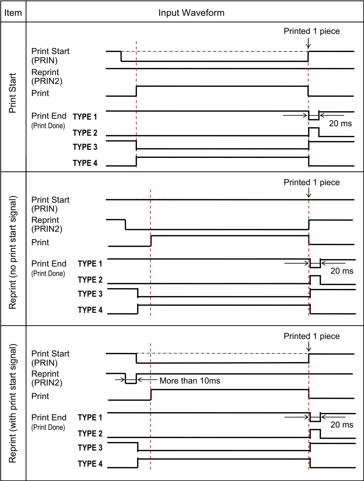
Timing Chart of the EXT Input Signal
