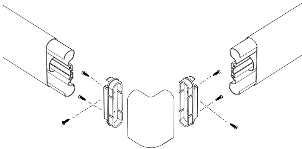
Corner Assembly
