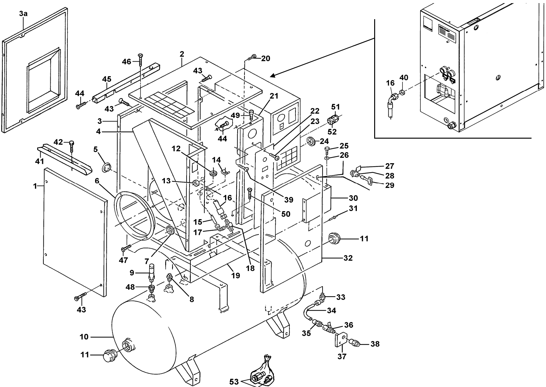
Dwg. 1 Casing - Sound-damping panels
