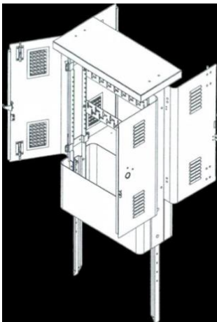
Stakes shown in mounting position. (During shipping stakes are mounted upside down within the cabinet)
