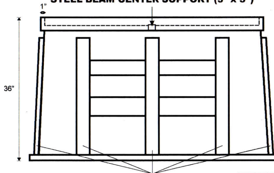
VERTICAL REINFORCEMENTS
