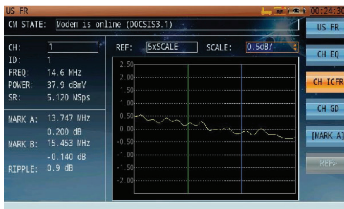
Figure 25: Get Upstream in-channel frequency response from the integrated DS2831 US Cable Modem.
