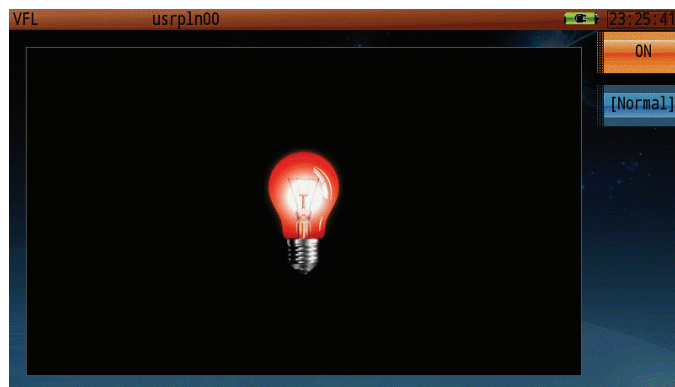
Figure 34: Check the fiber for continuity and detect damaged fibers or splices, including fiber breaks and excessive bends, with the Visual Fault Locator.
