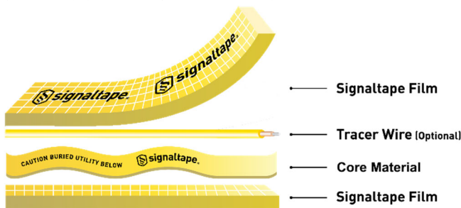
Figure 2 - Signaltape Construction
