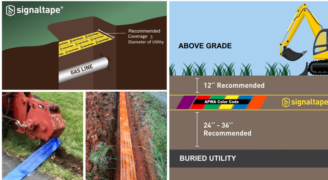
Figure 1 - Signaltape Installation
