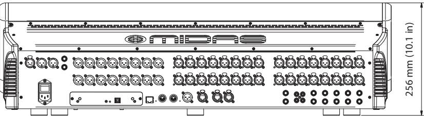
BACK VIEW
