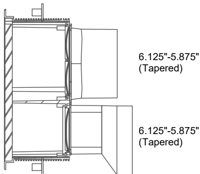
SECTIONAL SIDE VIEW
