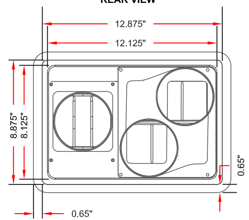
REAR VIEW
