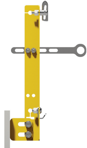
3 Single leg assembly with emergency pull cord eyelet
