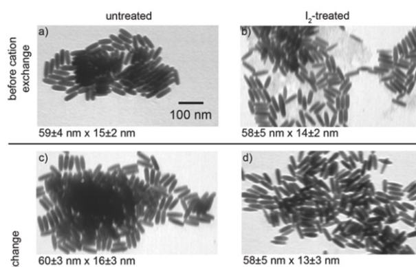
TEM of Cu 1.8 S nanorods synthesized by Dr. Plass’s group. (Le, 2020)
