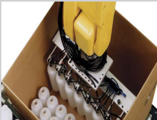
Case packing with Fanuc LR Mate
