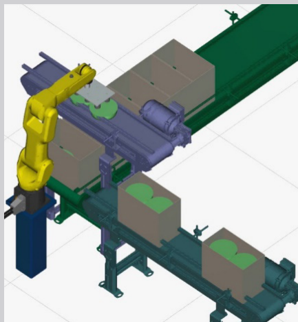
Robot simulations improve results
