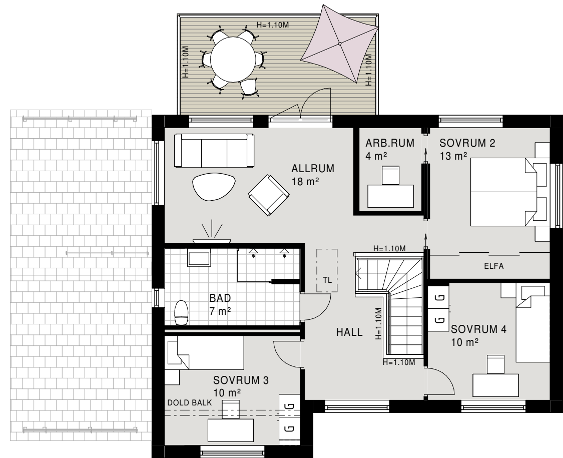
PLAN 2
