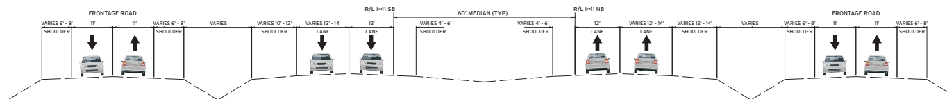
EXISTING TYPICAL SECTION - I-41 COUNTY J TO COUNTY F
